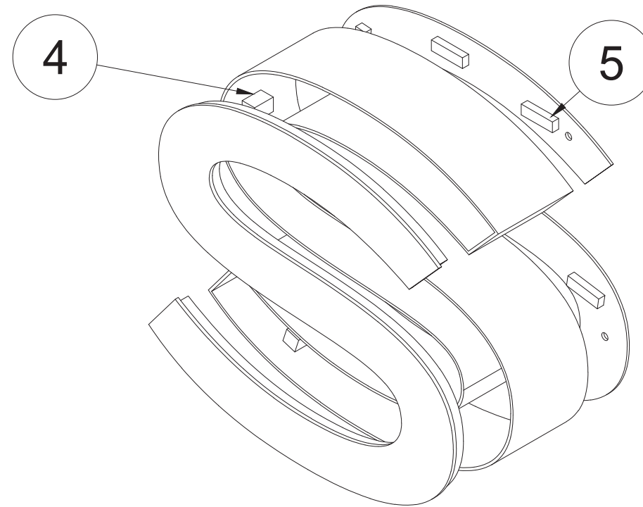
EXPLODED ISOMETRIC VIEW
